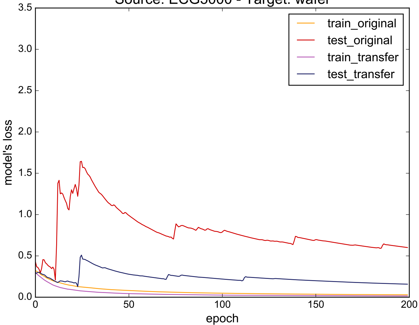
Source: ECG5000 - Target: wafer
