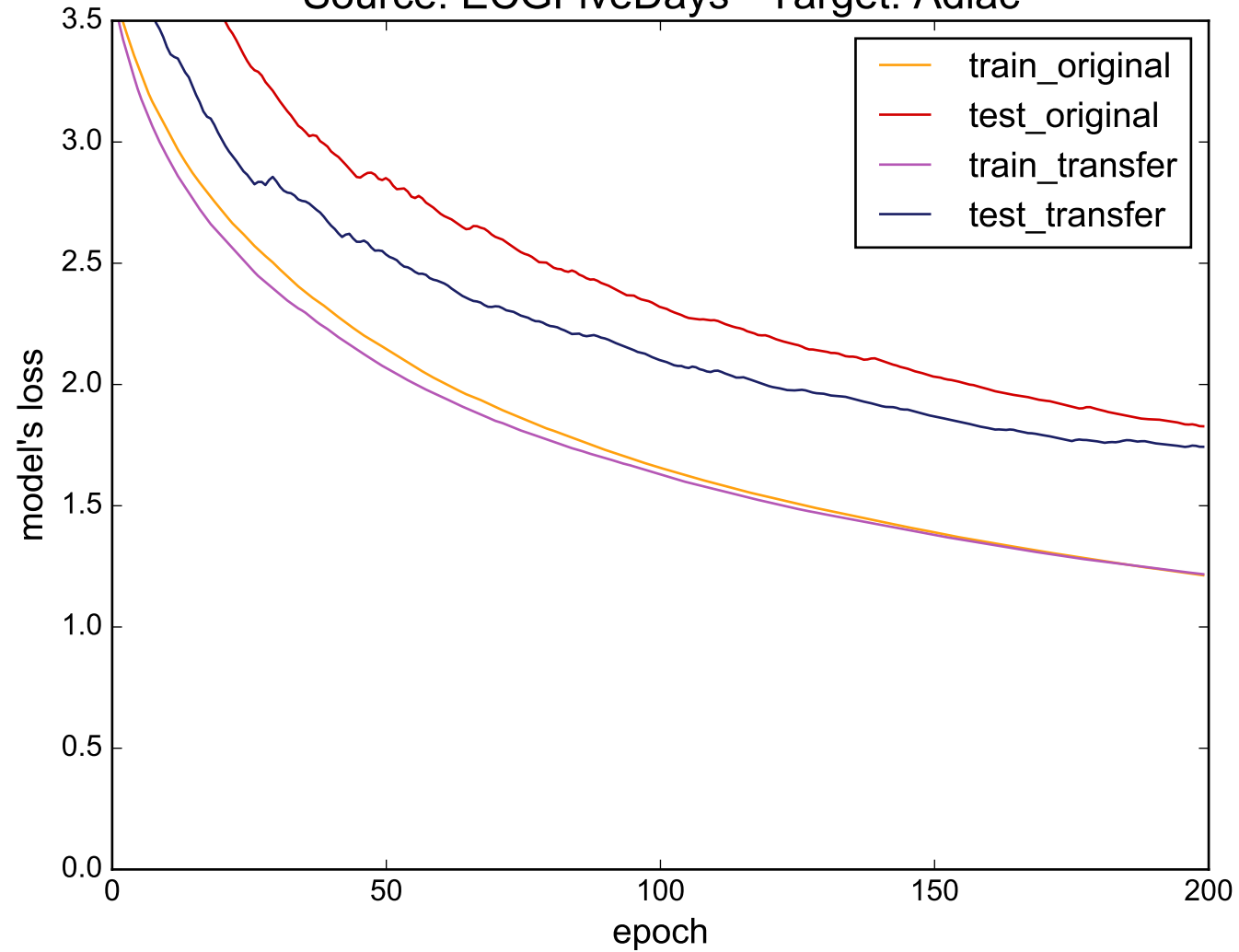
Source: ECGFiveDays - Target: Adiac
