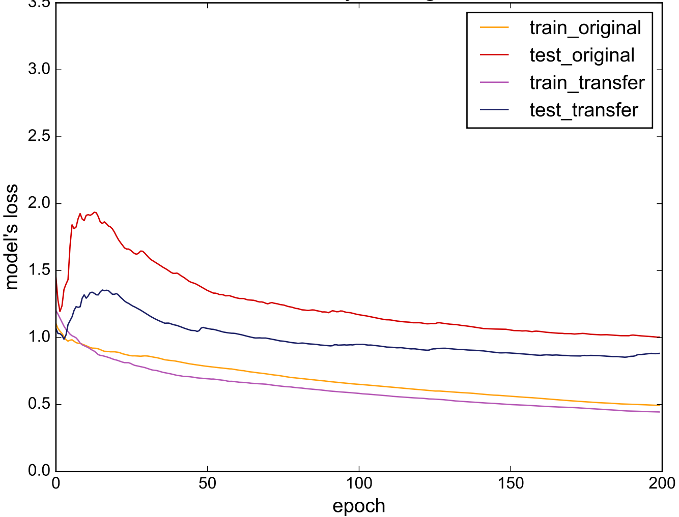
Source: ECGFiveDays - Target: ArrowHead
