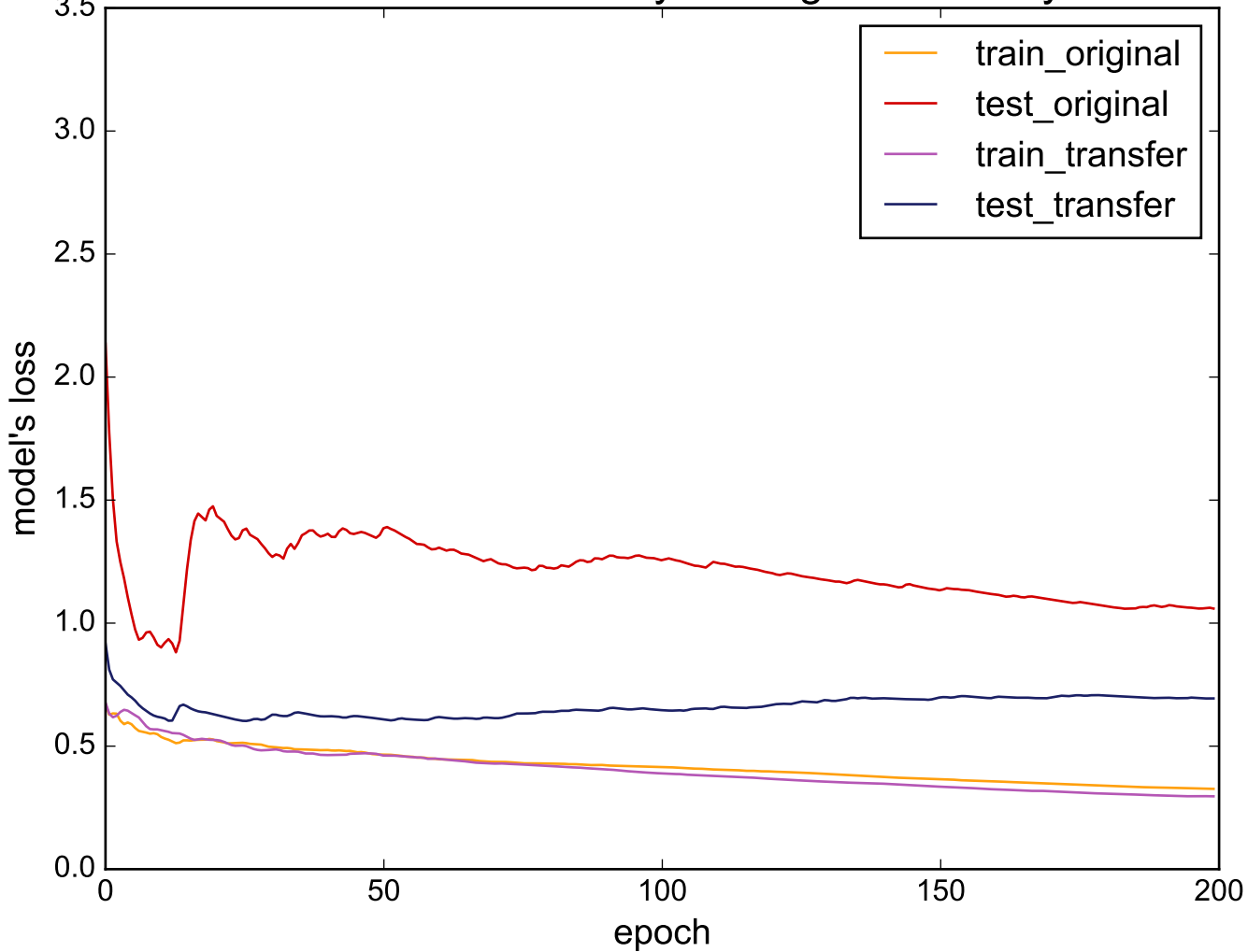
Source: ECGFiveDays - Target: BeetleFly
