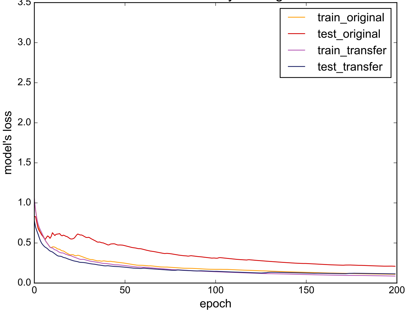
Source: ECGFiveDays - Target: CBF
