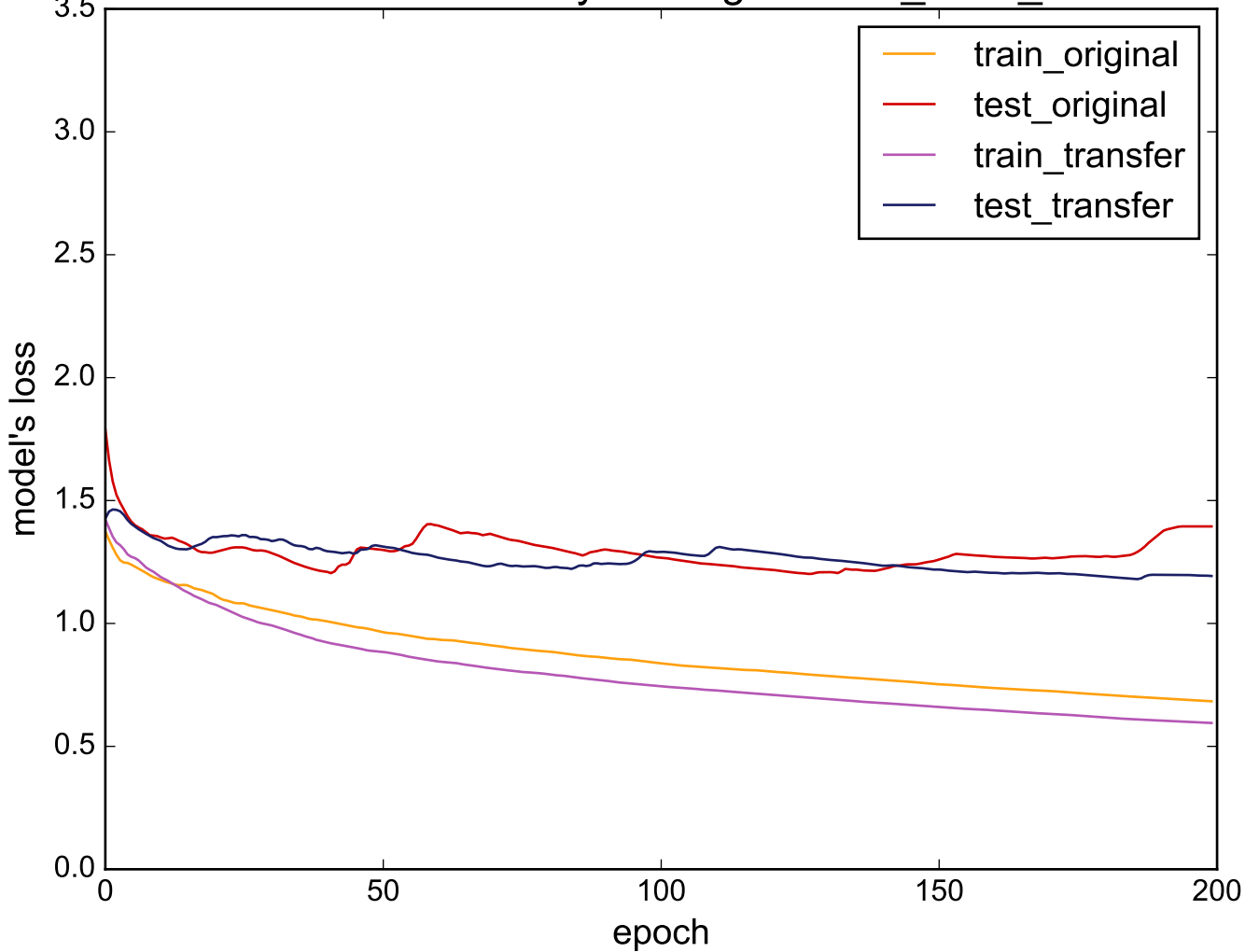
Source: ECGFiveDays - Target: CinC_ECG_torso
