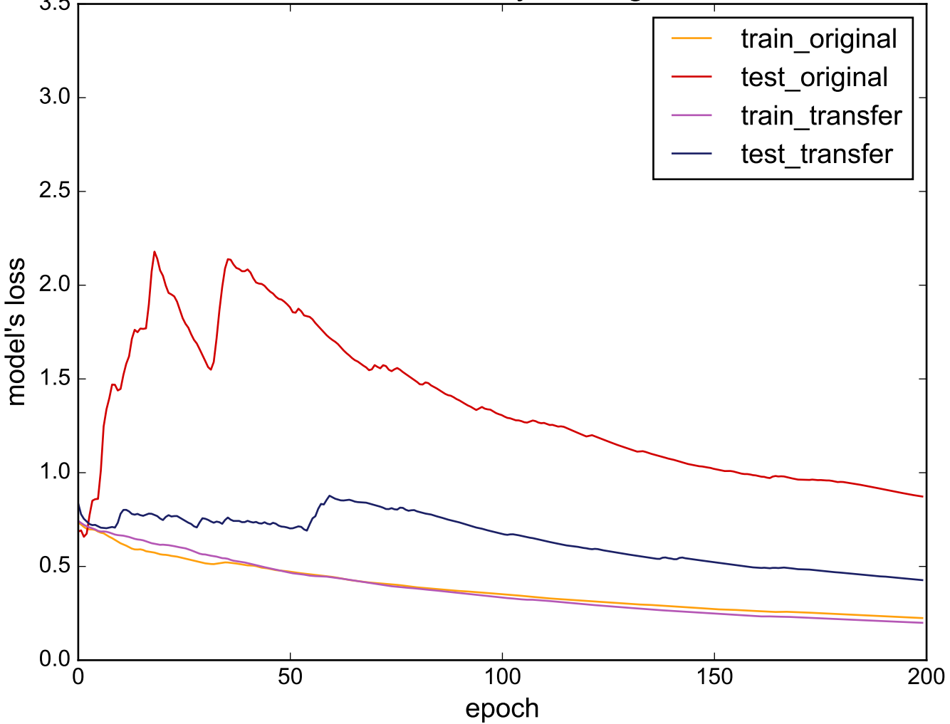
Source: ECGFiveDays - Target: Coffee
