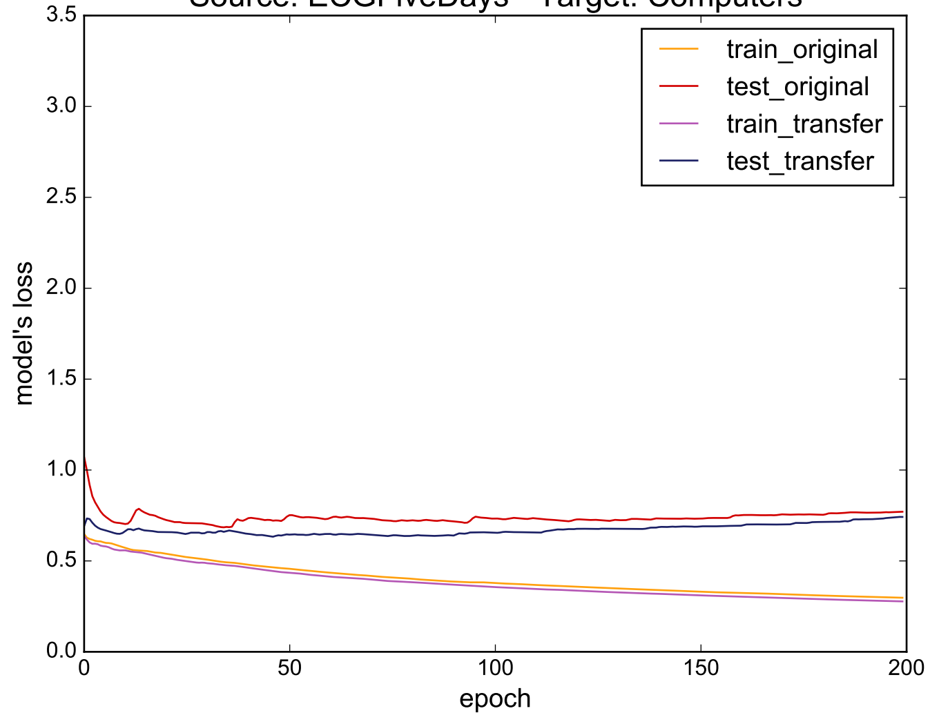
Source: ECGFiveDays - Target: Computers
