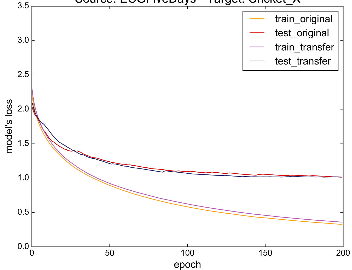
Source: ECGFiveDays - Target: Cricket_X
