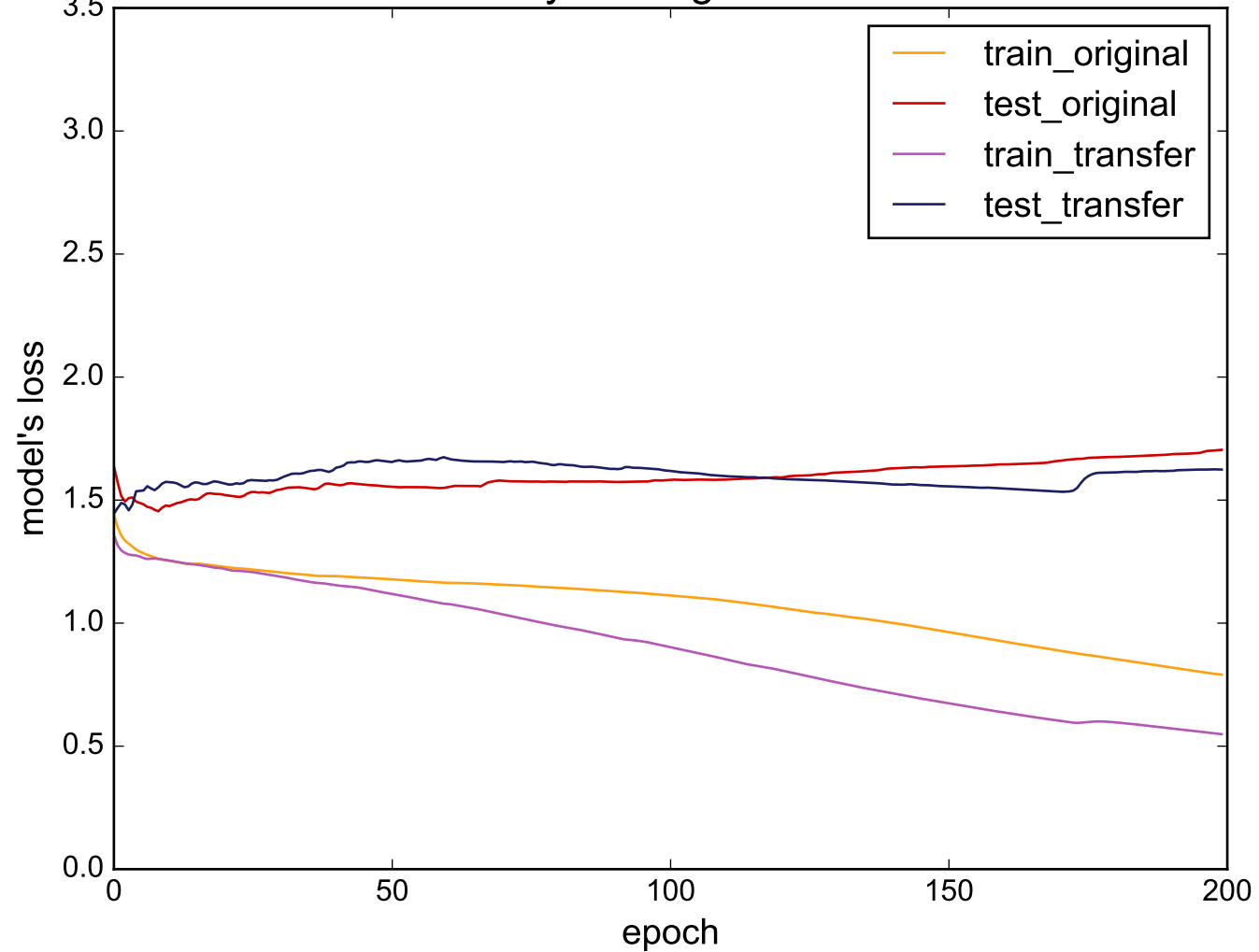
Source: ECGFiveDays - Target: DiatomSizeReduction
