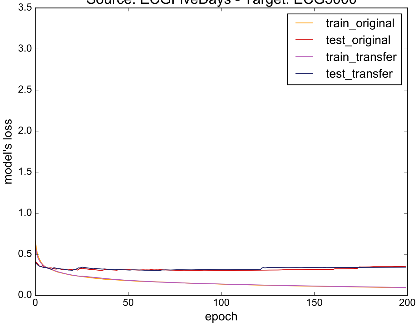
Source: ECGFiveDays - Target: ECG5000
