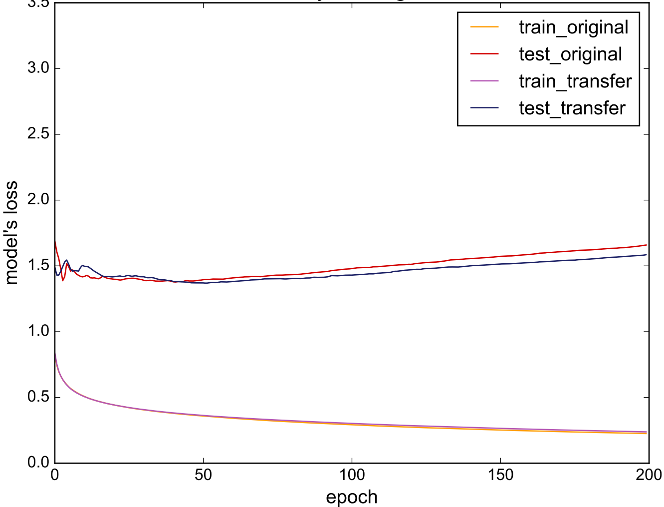
Source: ECGFiveDays - Target: ElectricDevices
