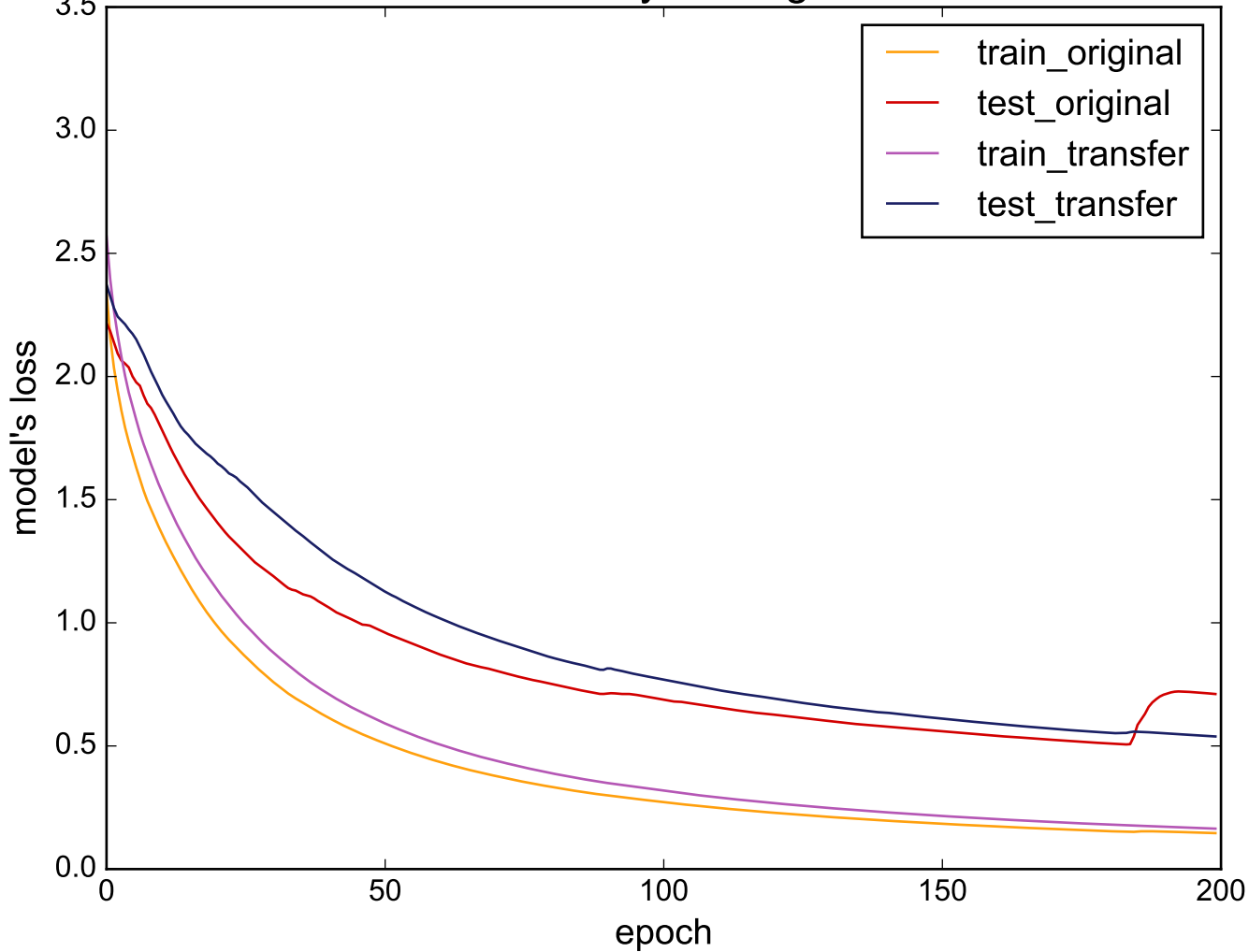
Source: ECGFiveDays - Target: FacesUCR
