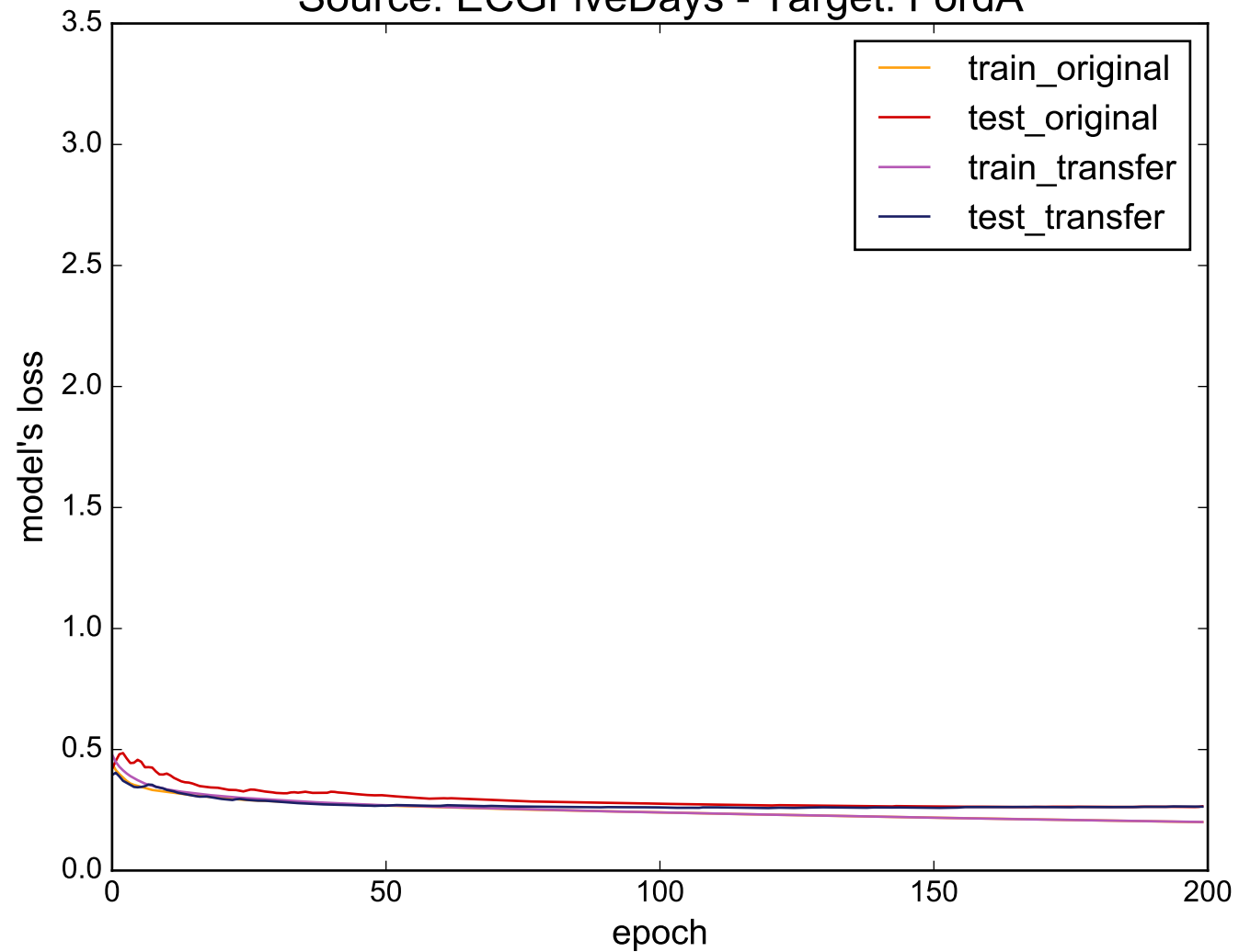
Source: ECGFiveDays - Target: FordA
