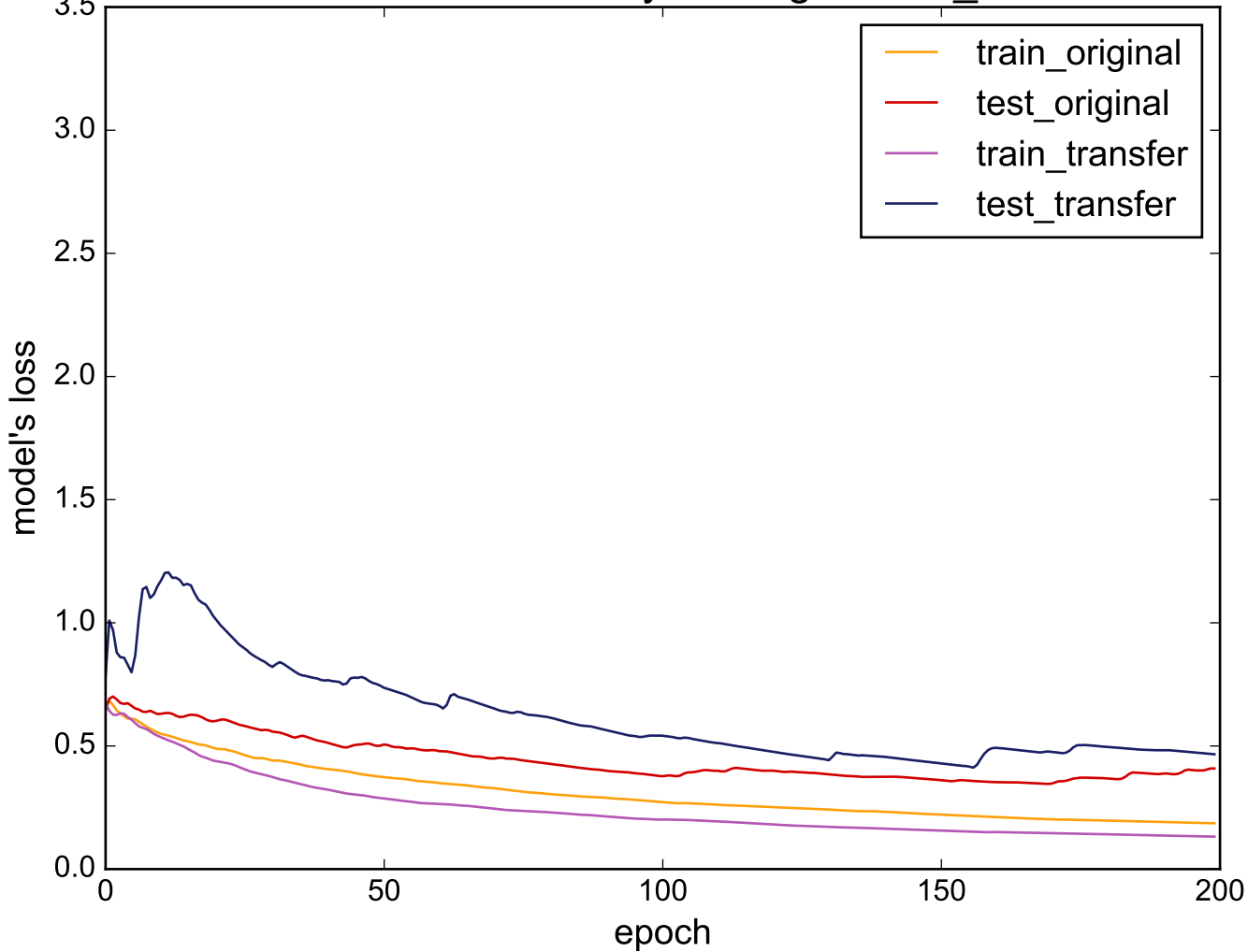
Source: ECGFiveDays - Target: Gun_Point
