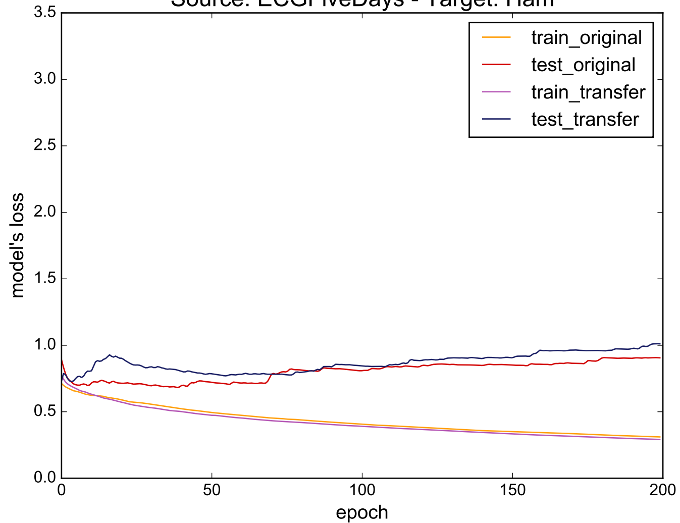
Source: ECGFiveDays - Target: Ham
