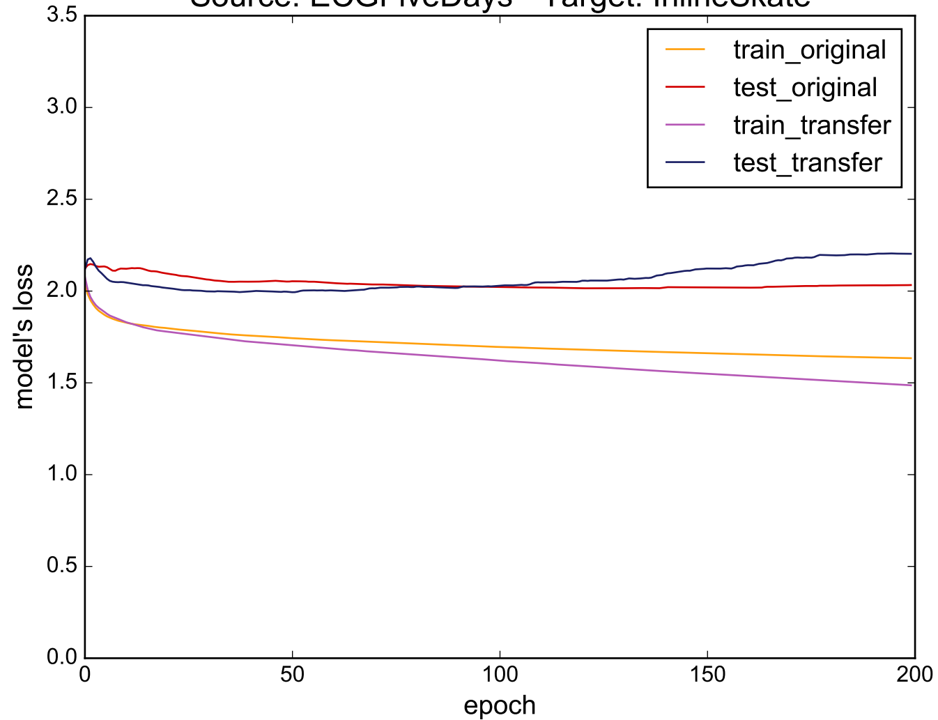
Source: ECGFiveDays - Target: InlineSkate
