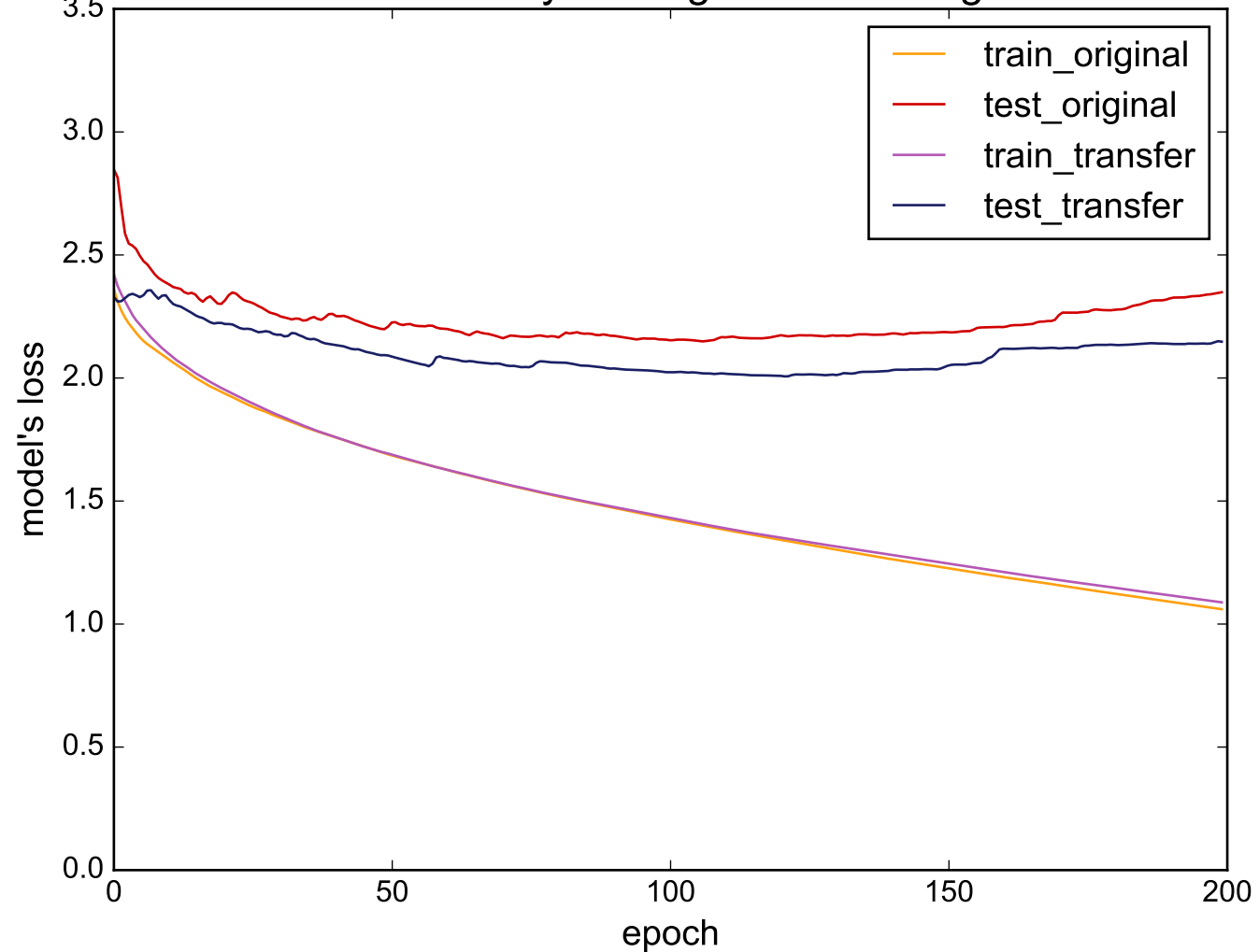
Source: ECGFiveDays - Target: InsectWingbeatSound
