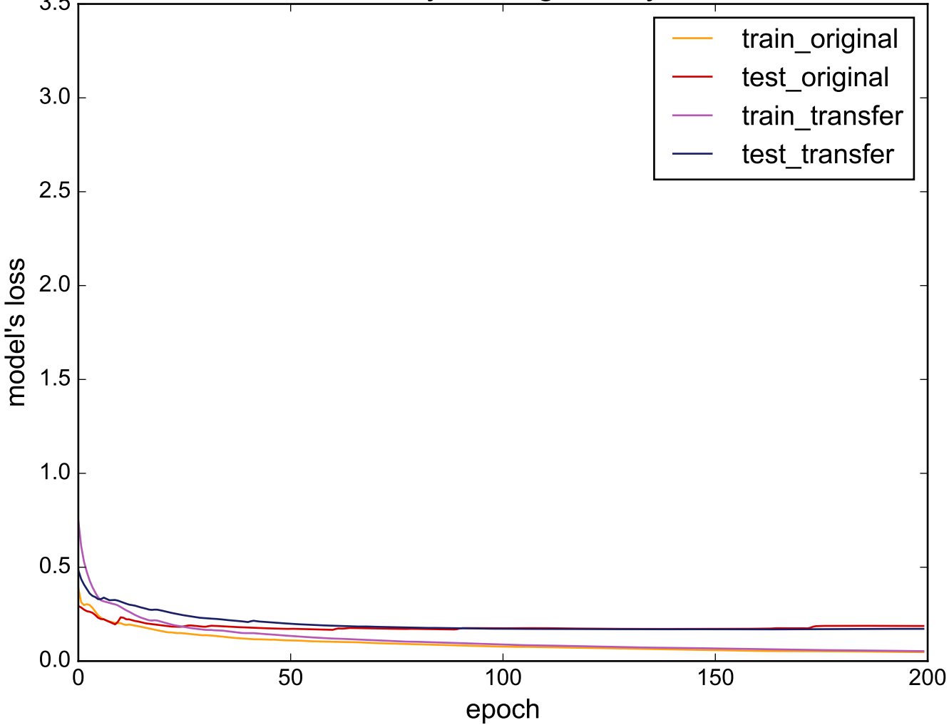
Source: ECGFiveDays - Target: ItalyPowerDemand
