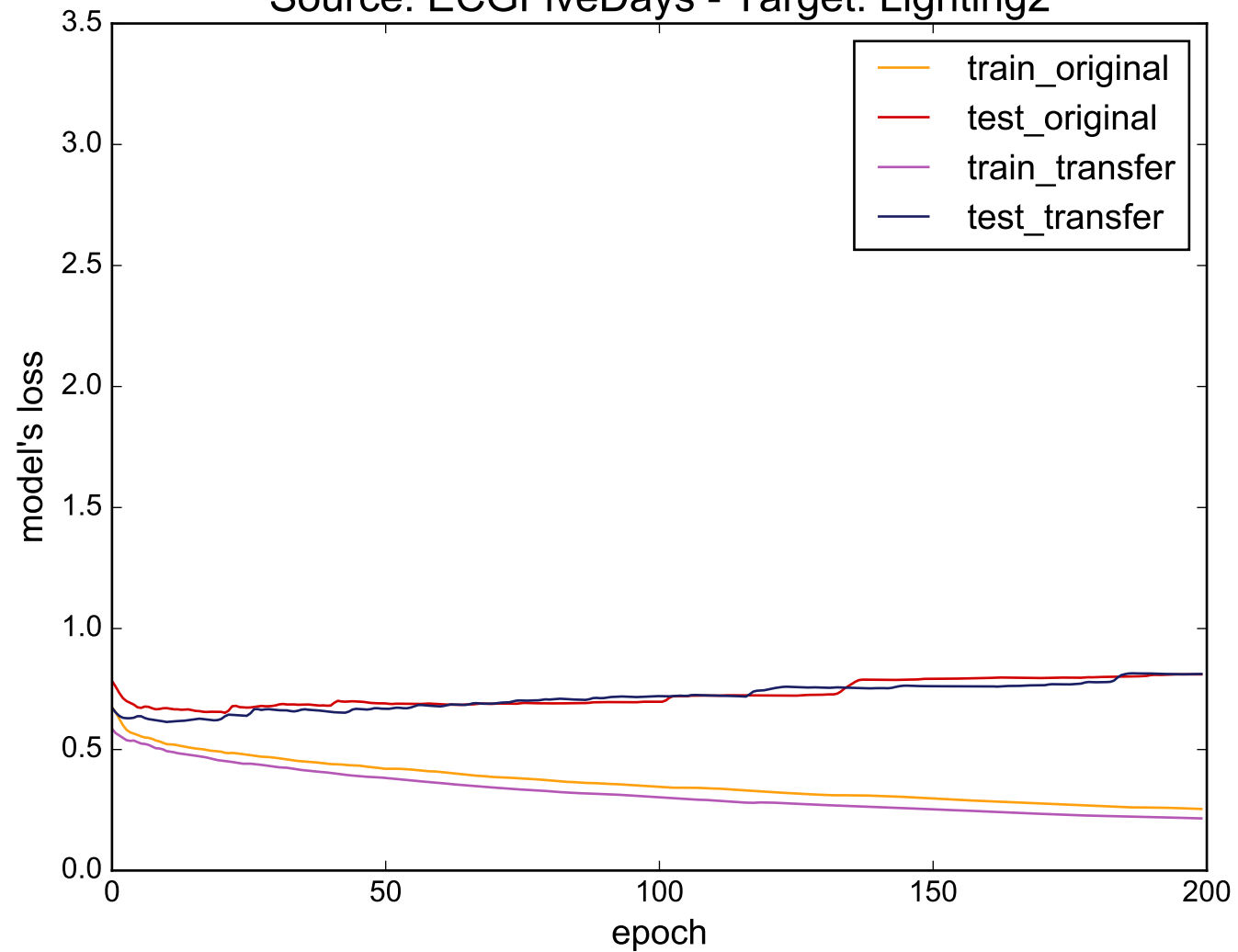
Source: ECGFiveDays - Target: Lighting2
