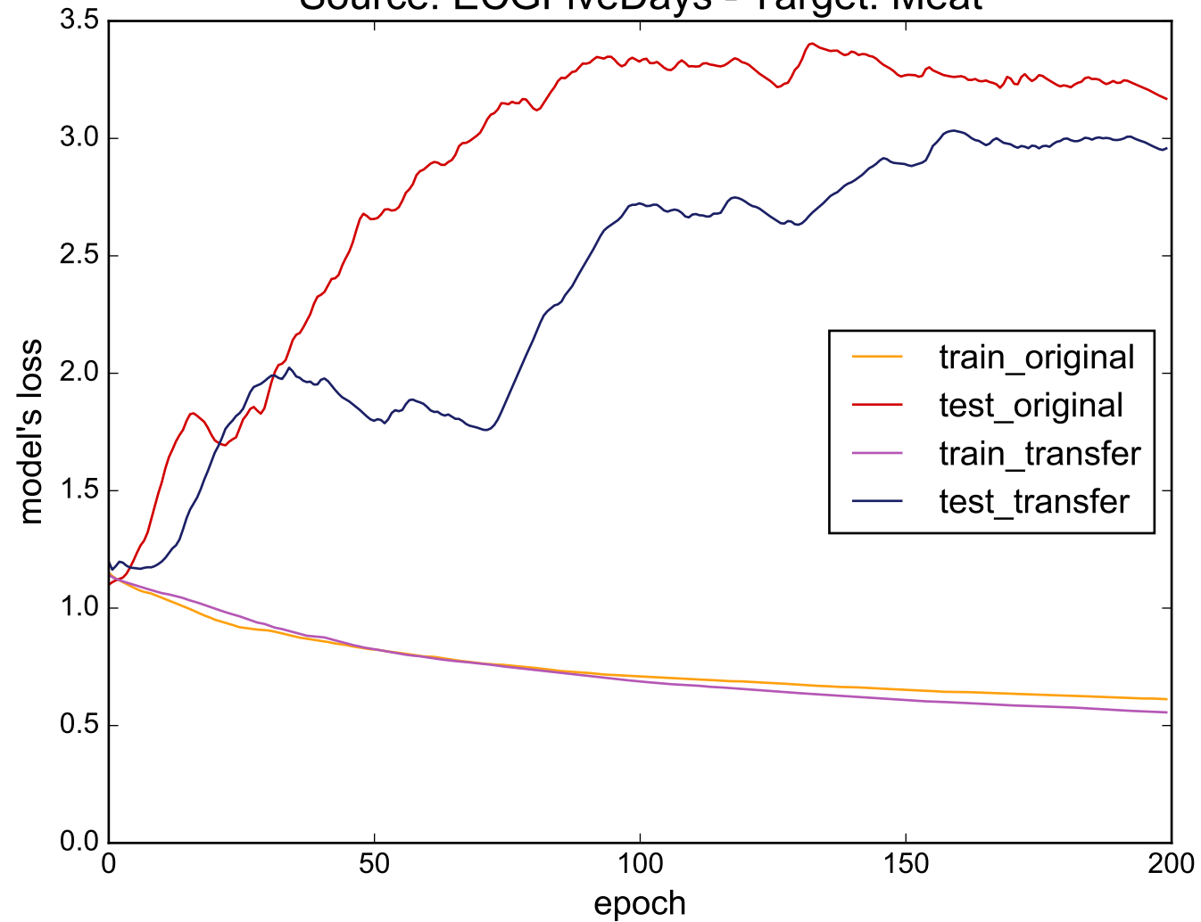
Source: ECGFiveDays - Target: Meat
