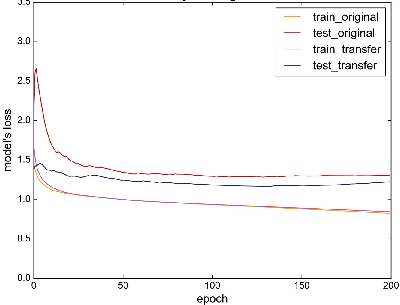
Source: ECGFiveDays - Target: MiddlePhalanxTW
