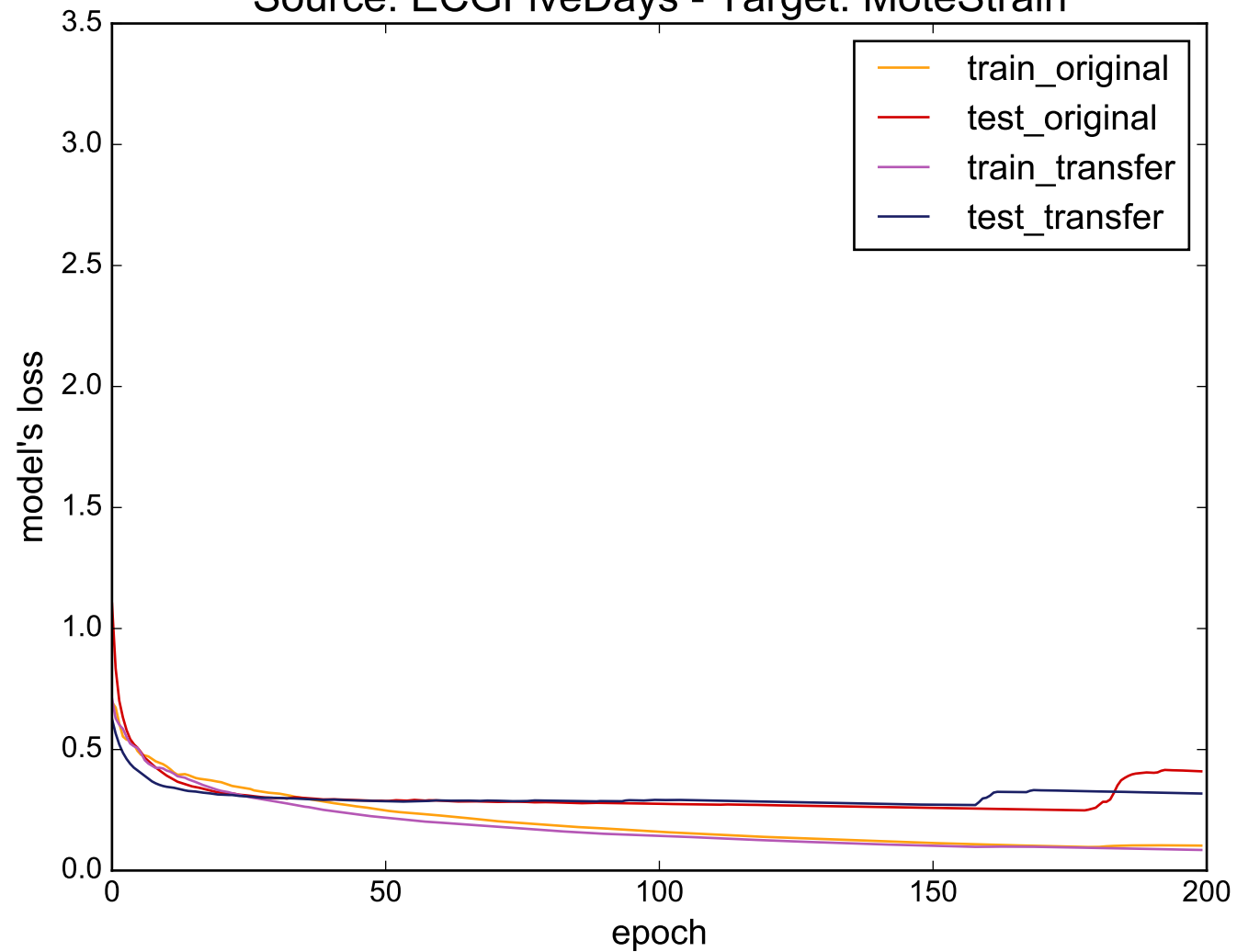
Source: ECGFiveDays - Target: MoteStrain
