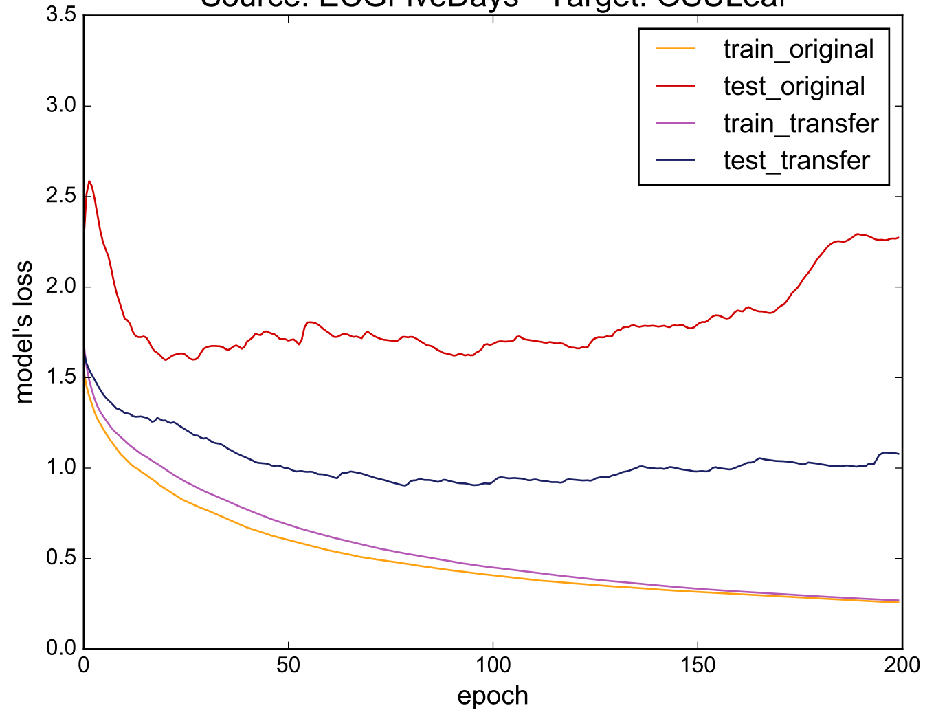
Source: ECGFiveDays - Target: OSULeaf
