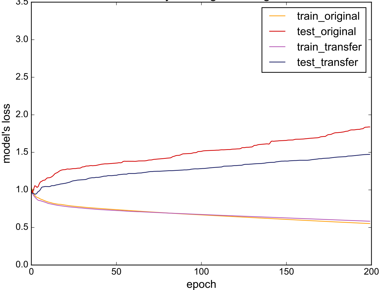
Source: ECGFiveDays - Target: RefrigerationDevices
