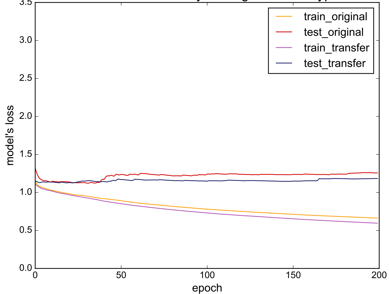
Source: ECGFiveDays - Target: ScreenType
