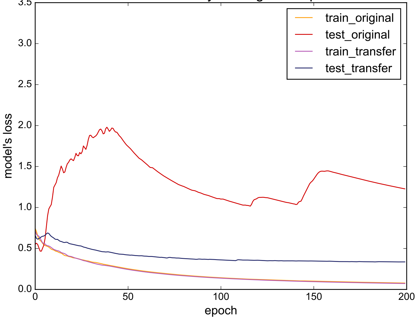
Source: ECGFiveDays - Target: ShapeletSim
