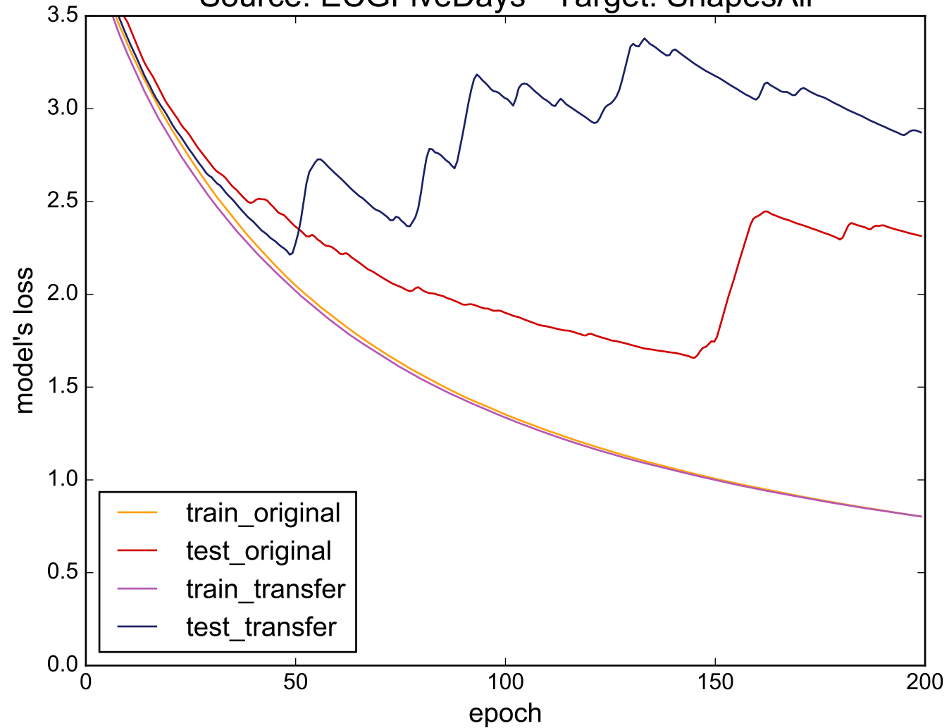
Source: ECGFiveDays - Target: ShapesAll
