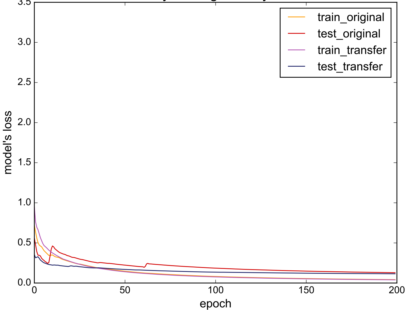
Source: ECGFiveDays - Target: SonyAIBORobotSurfaceII
