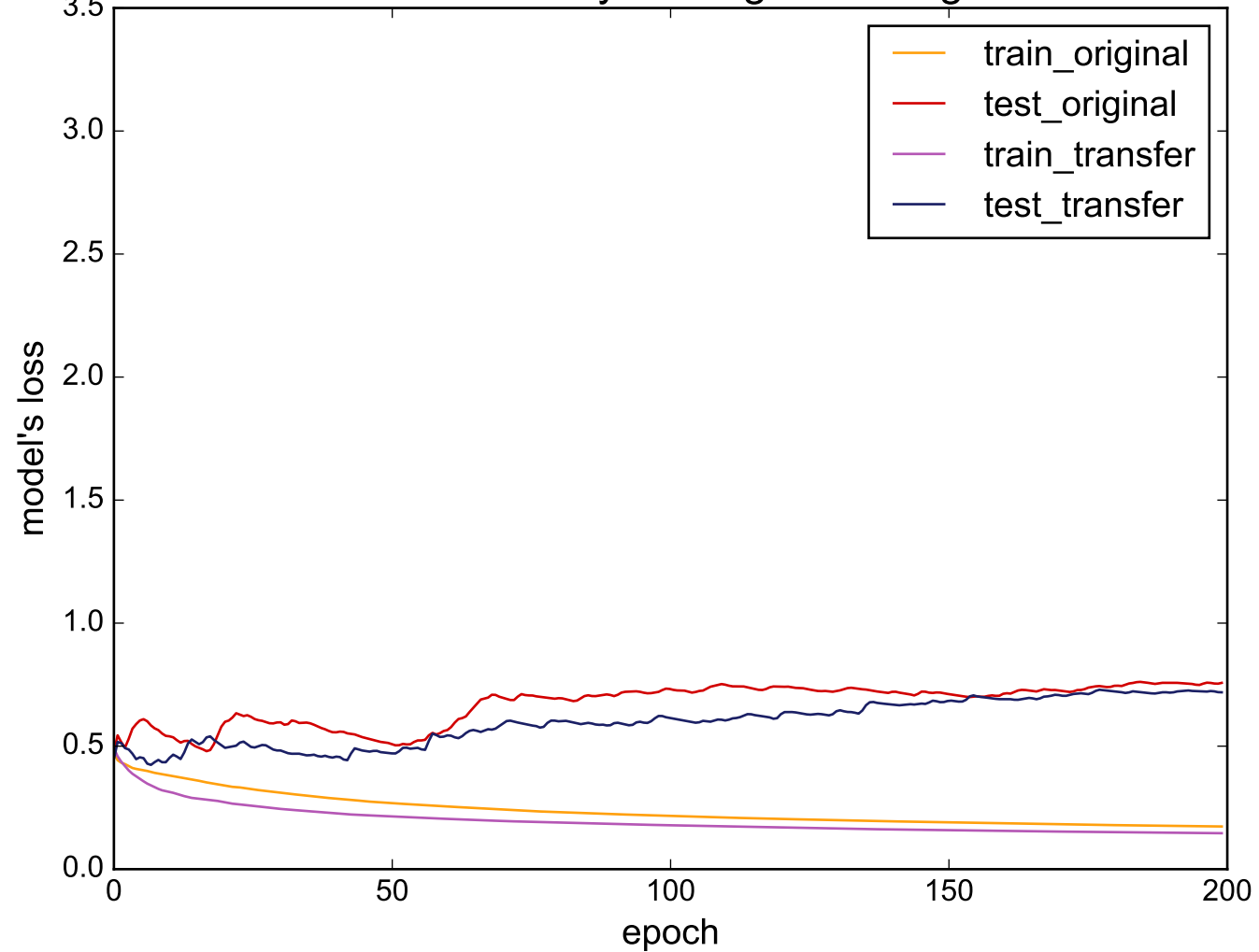
Source: ECGFiveDays - Target: StarLightCurves
