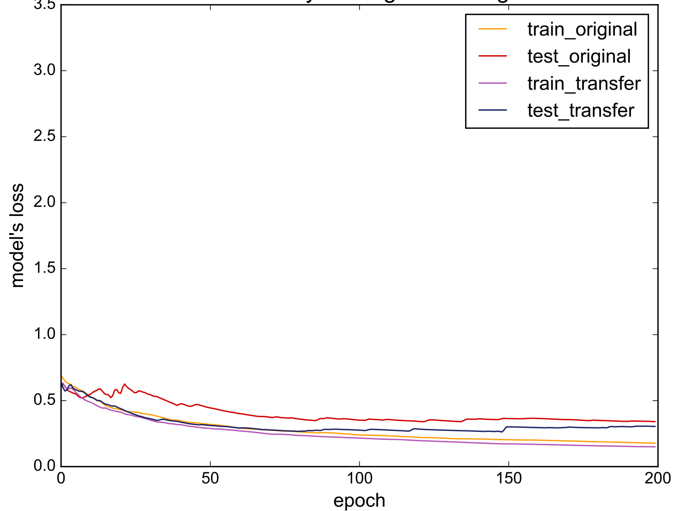
Source: ECGFiveDays - Target: ToeSegmentation1
