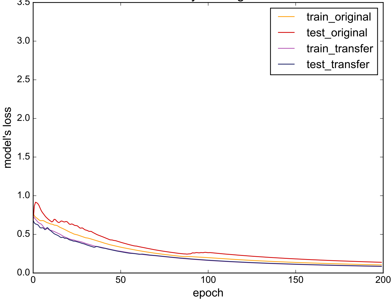
Source: ECGFiveDays - Target: TwoLeadECG
