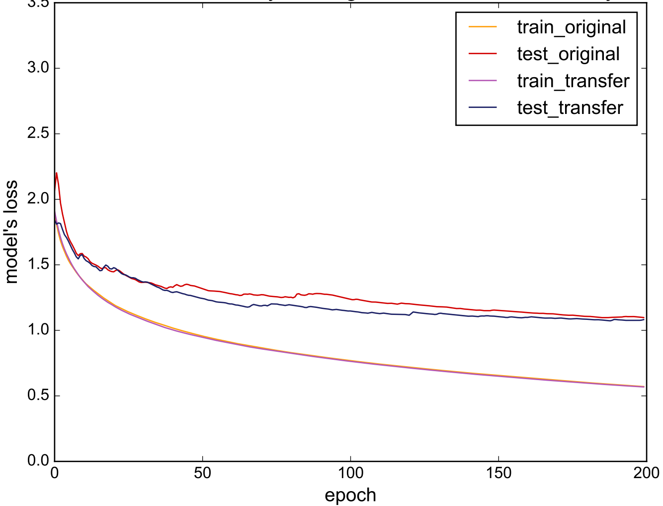
Source: ECGFiveDays - Target: UWaveGestureLibraryAll
