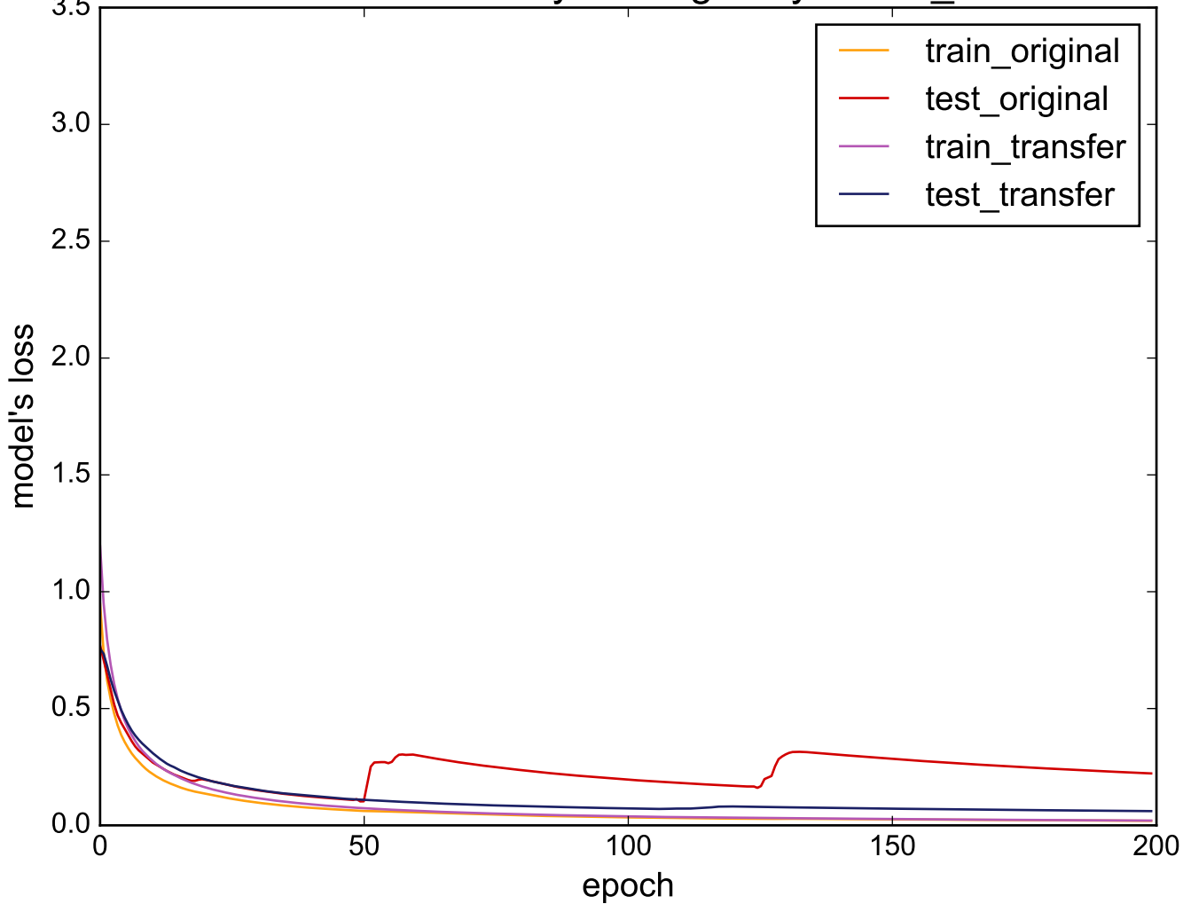
Source: ECGFiveDays - Target: synthetic_control
