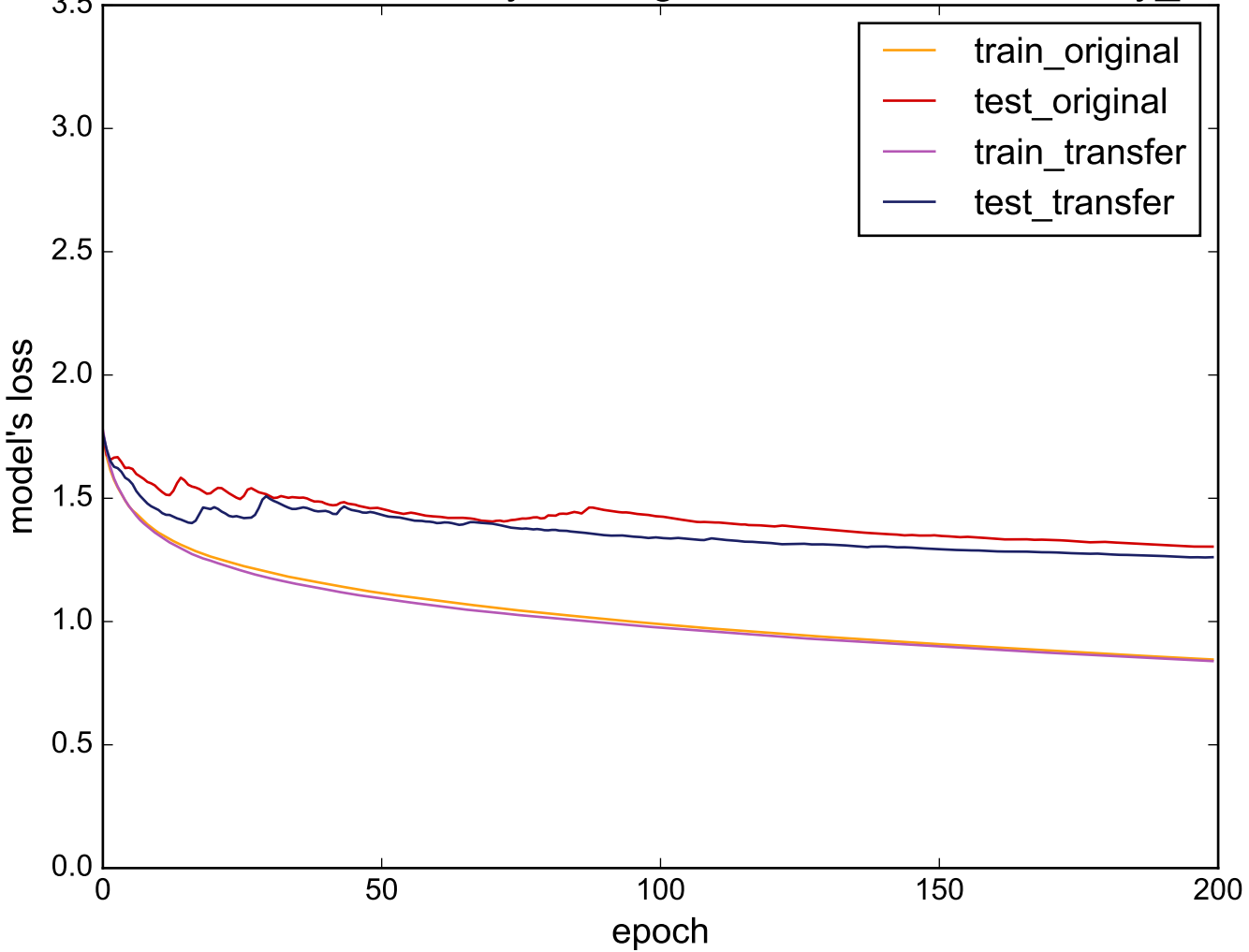
Source: ECGFiveDays - Target: uWaveGestureLibrary_Y
