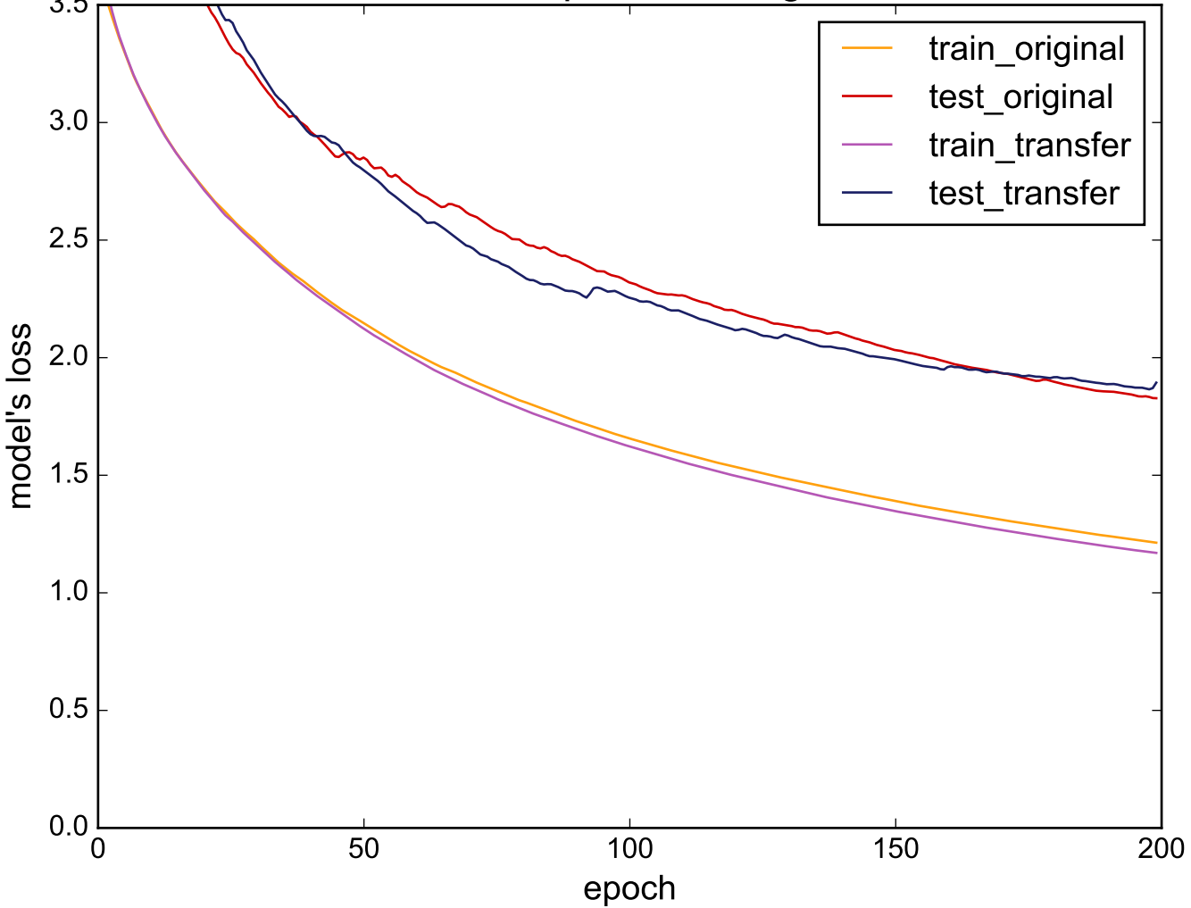
Source: Earthquakes - Target: Adiac
