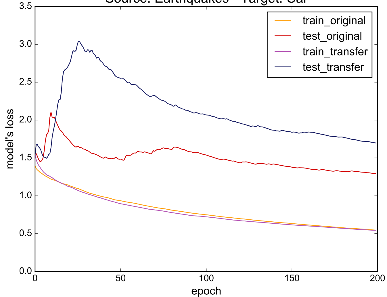
Source: Earthquakes - Target: Car
