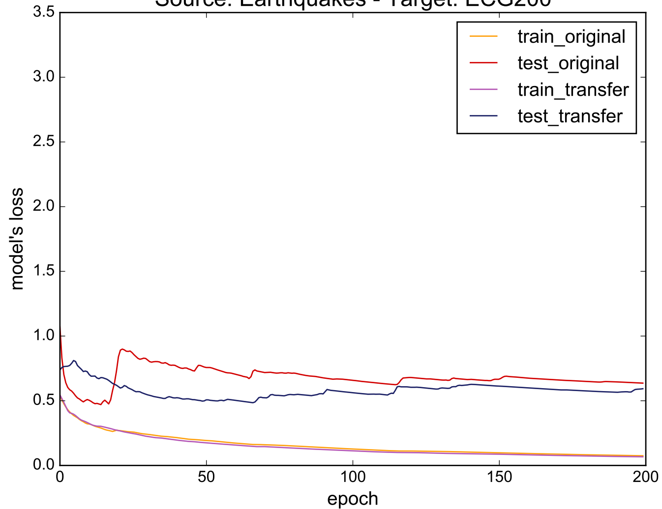
Source: Earthquakes - Target: ECG200
