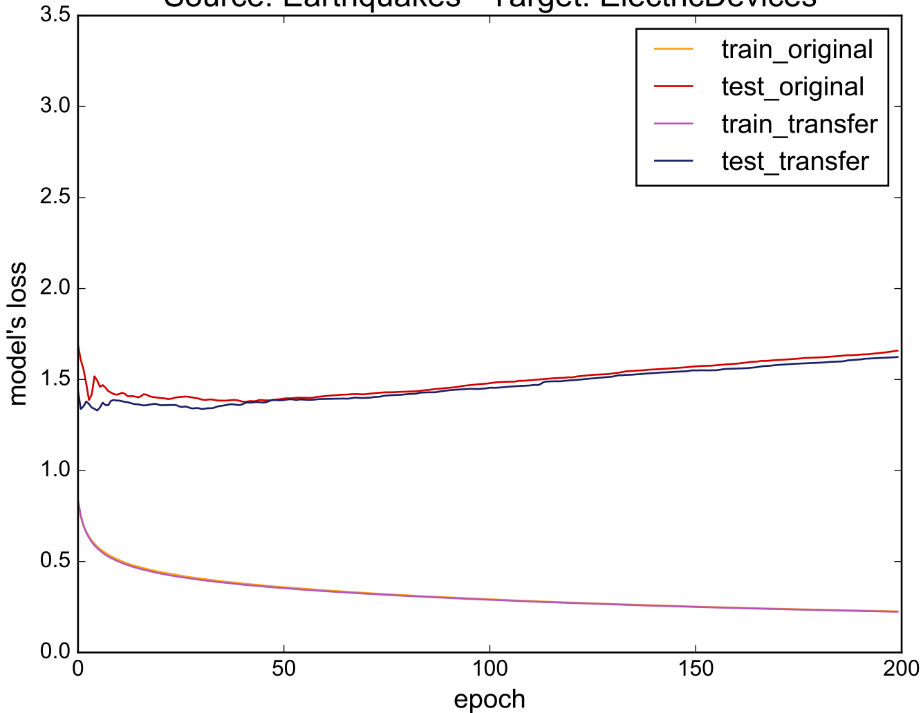
Source: Earthquakes - Target: ElectricDevices
