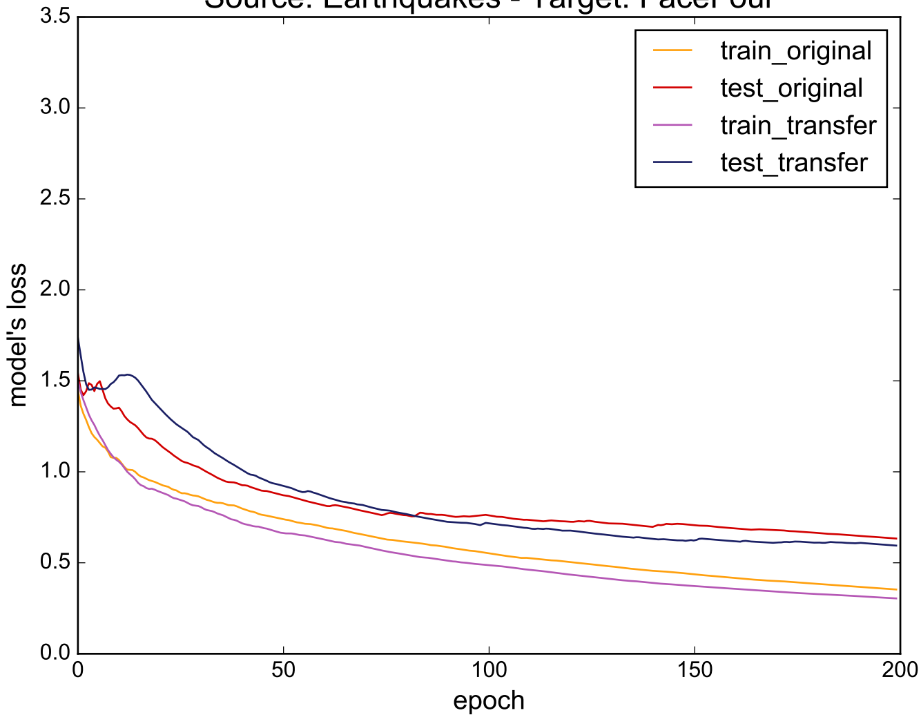
Source: Earthquakes - Target: FaceFour
