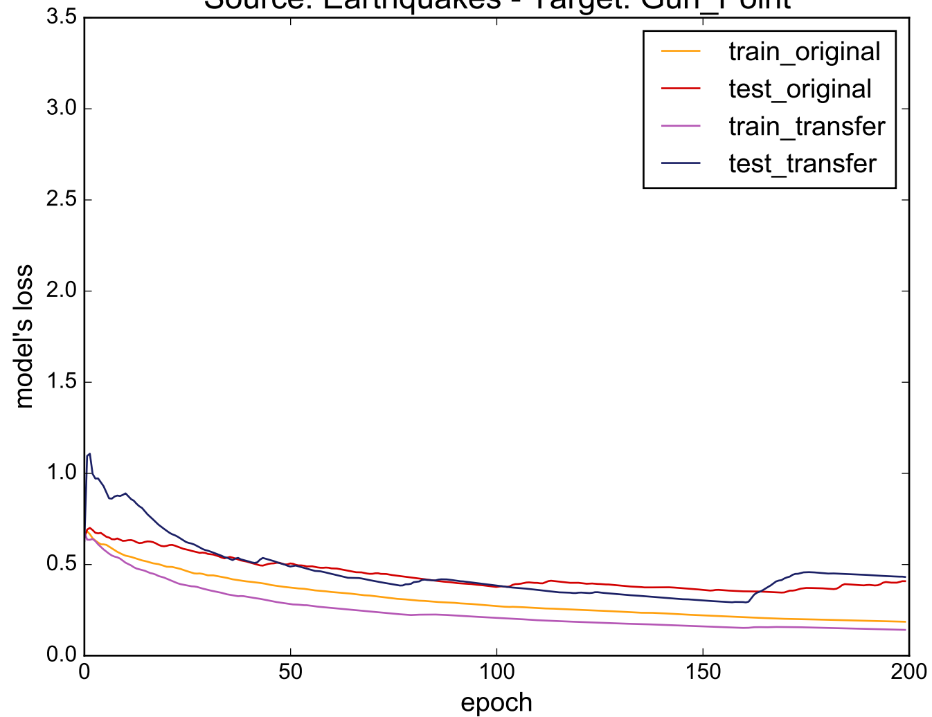
Source: Earthquakes - Target: Gun_Point
