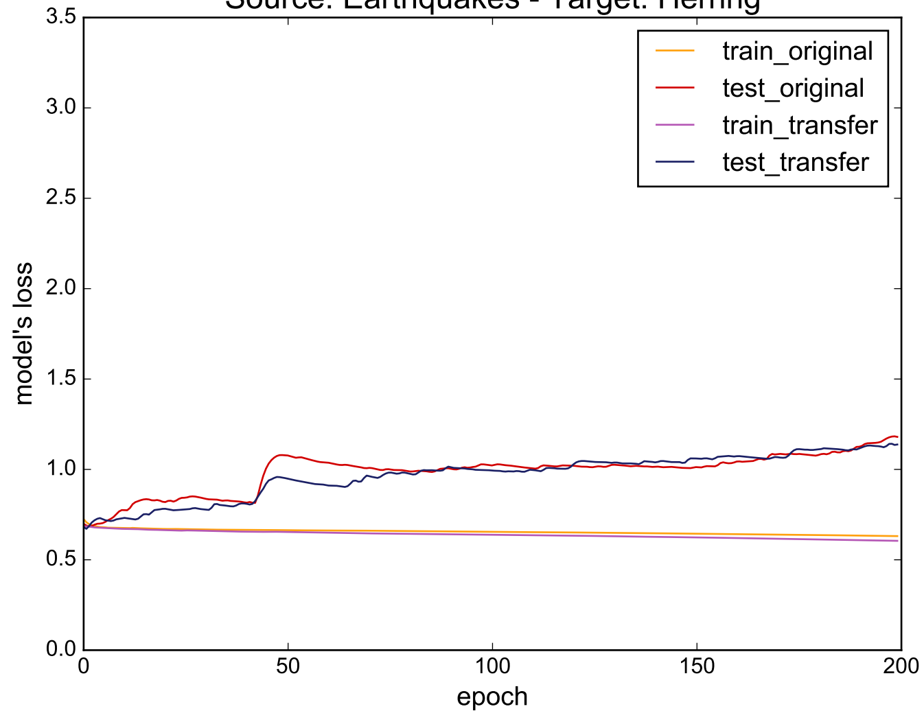
Source: Earthquakes - Target: Herring
