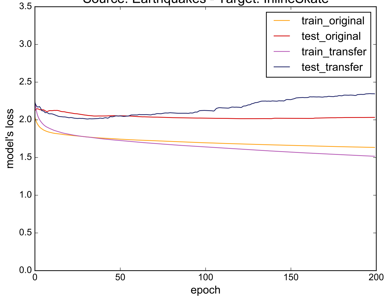
Source: Earthquakes - Target: InlineSkate
