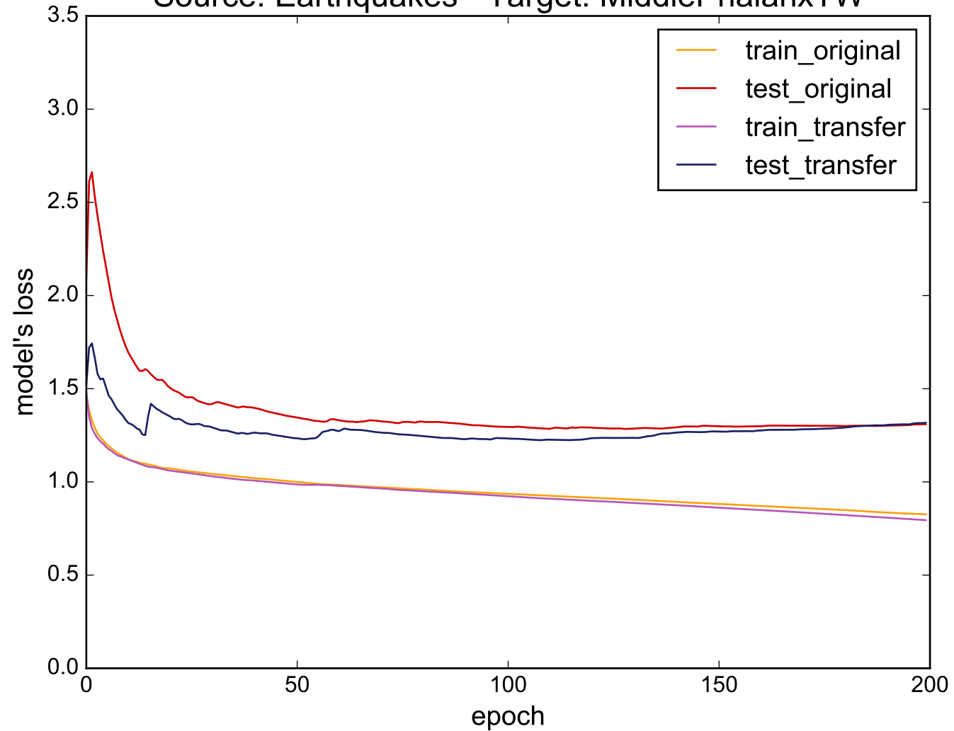
Source: Earthquakes - Target: MiddlePhalanxTW
