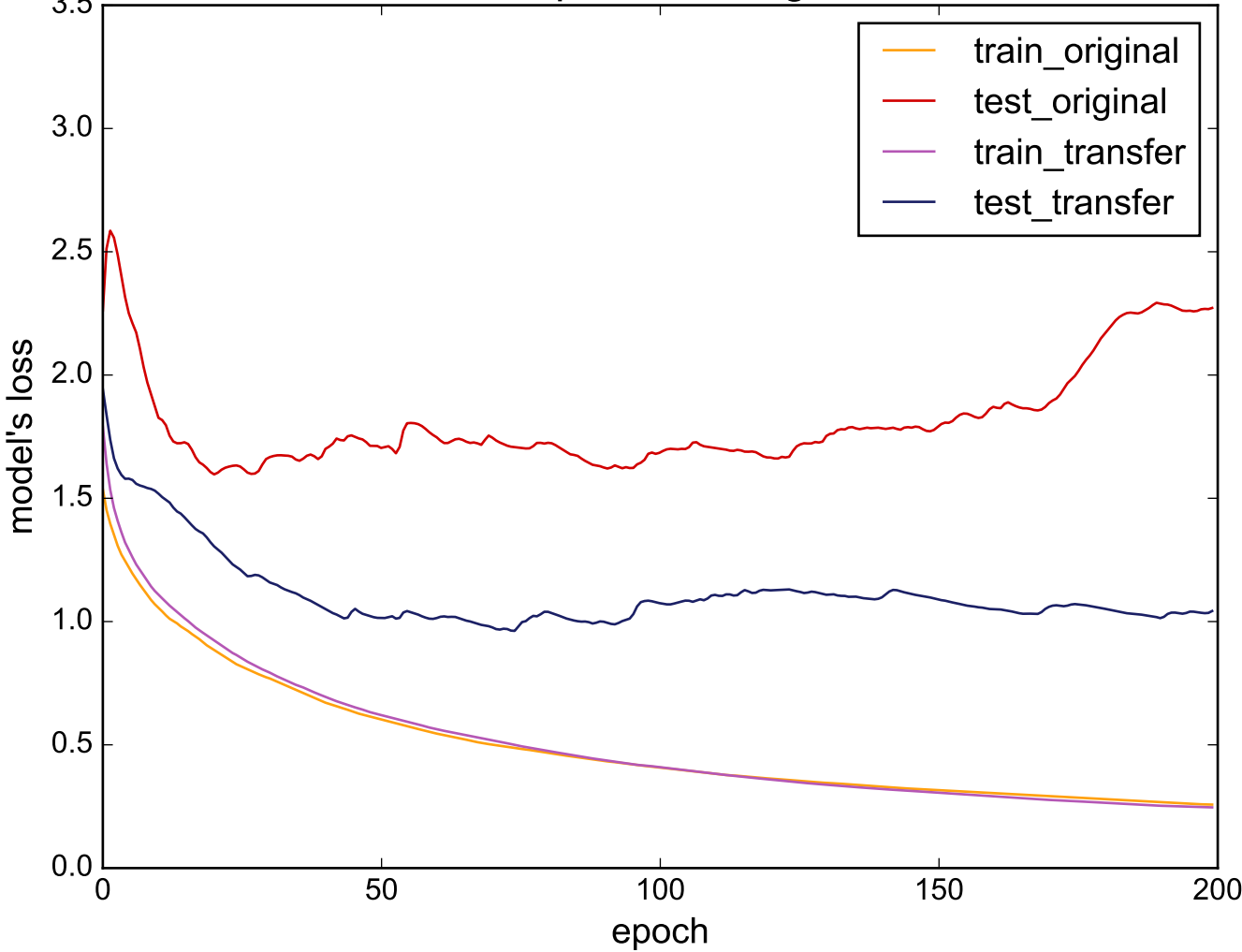
Source: Earthquakes - Target: OSULeaf
