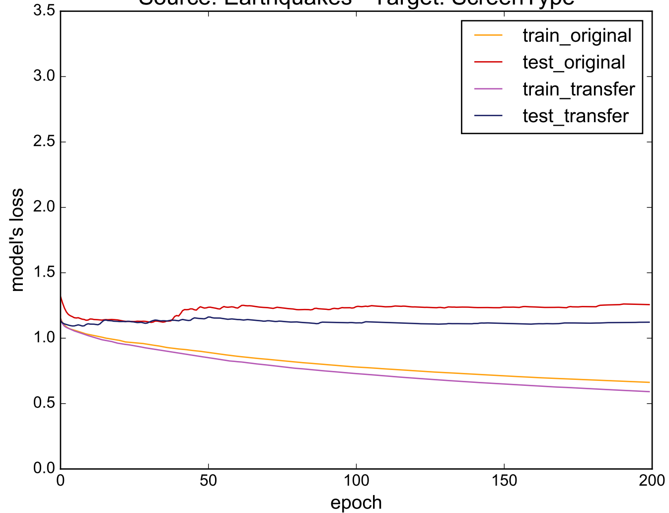
Source: Earthquakes - Target: ScreenType
