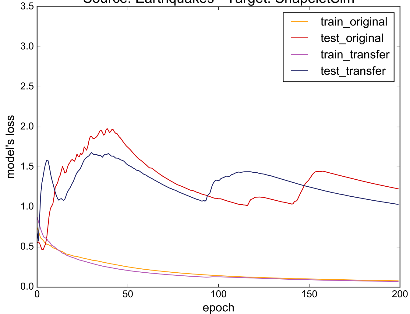
Source: Earthquakes - Target: ShapeletSim
