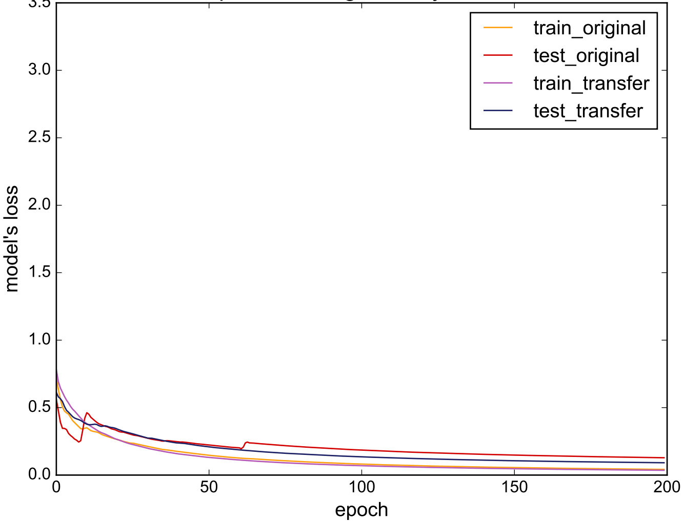
Source: Earthquakes - Target: SonyAIBORobotSurfacell
