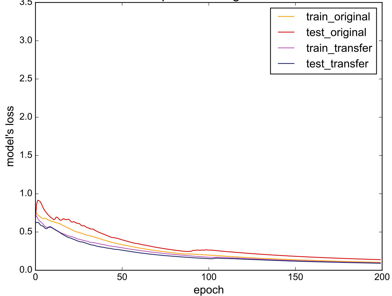
Source: Earthquakes - Target: TwoLeadECG
