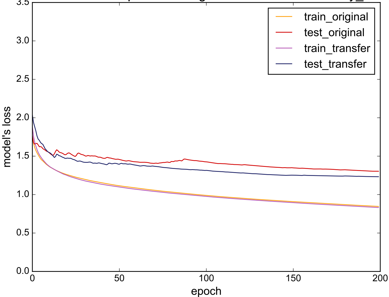
Source: Earthquakes - Target: uWaveGestureLibrary_Y
